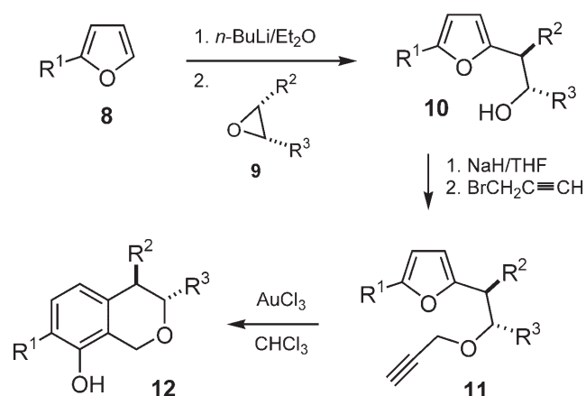
Scheme 4. Ring-opening of oxiranes as the basis for the synthesis of isochromanes 12 .
