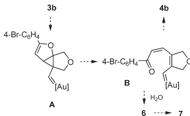
Scheme 3. Echavarren's mechanistic suggestion for the formation of side-products of type 6 .
