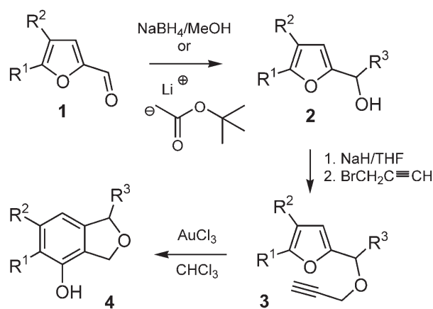
Scheme 1. Nucleophilic additions to furfural derivatives as the basis for the synthesis of dihydroisobenzofurans 4 .
