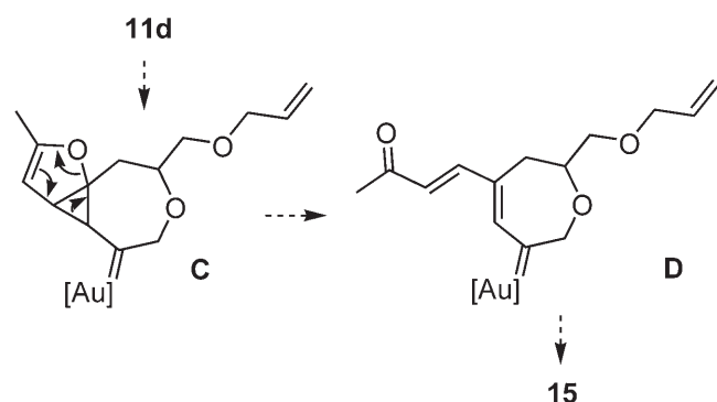
Scheme 6. Possible explanation for the formation of 15 .
