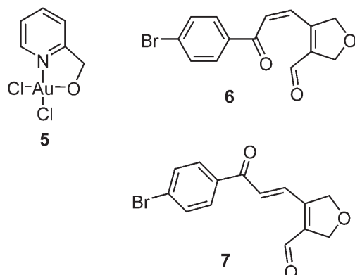
Scheme 2. Side-products 6 and 7 obtained from 2b with catalyst 5 .
