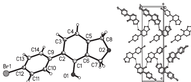
Figure 1. Structure of 3b and hydrogen intramolecular hydrogen bonding of the phenolic hydroxy group. [12]
