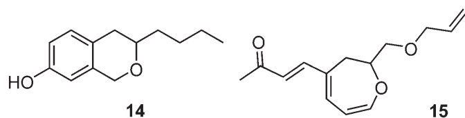
Scheme 5. Side-products 14 and 15 observed in the formation of isochromanes.
